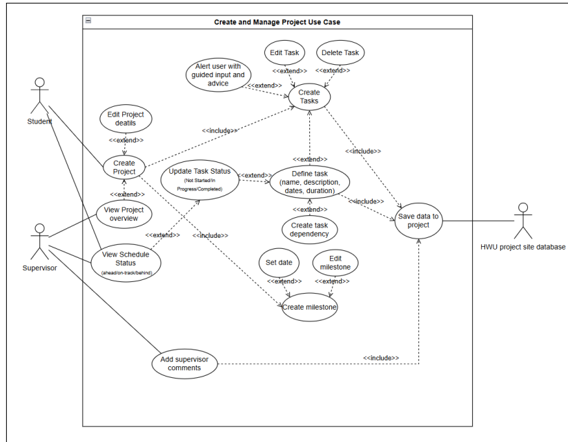
Fig. 1. Create and Manage Project Use Case Diagram.
